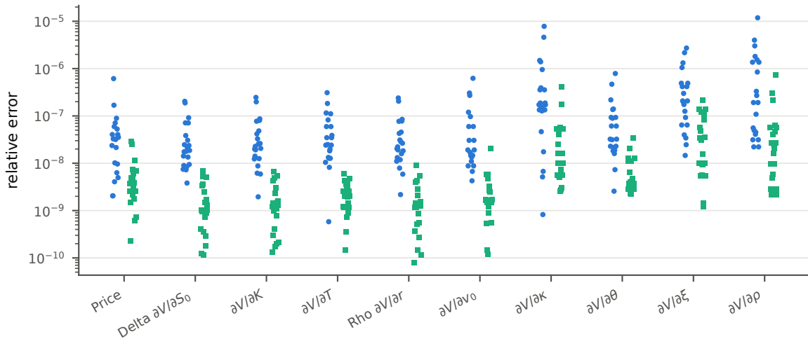
Generated shared-multiplier datapaths vs double-precision COS, 21 parameter sets
